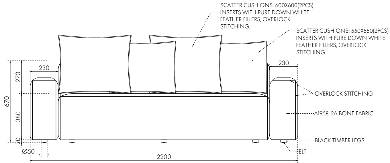
FRONT VIEW
