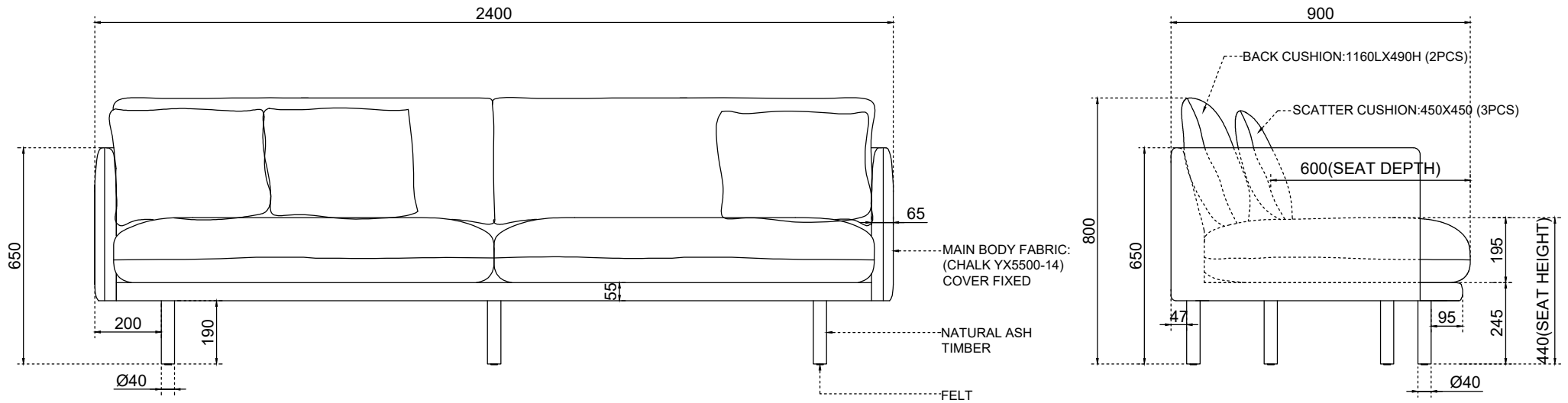
FRONT VIEW
