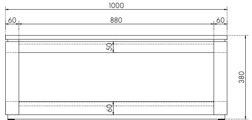
SIDE VIEW
